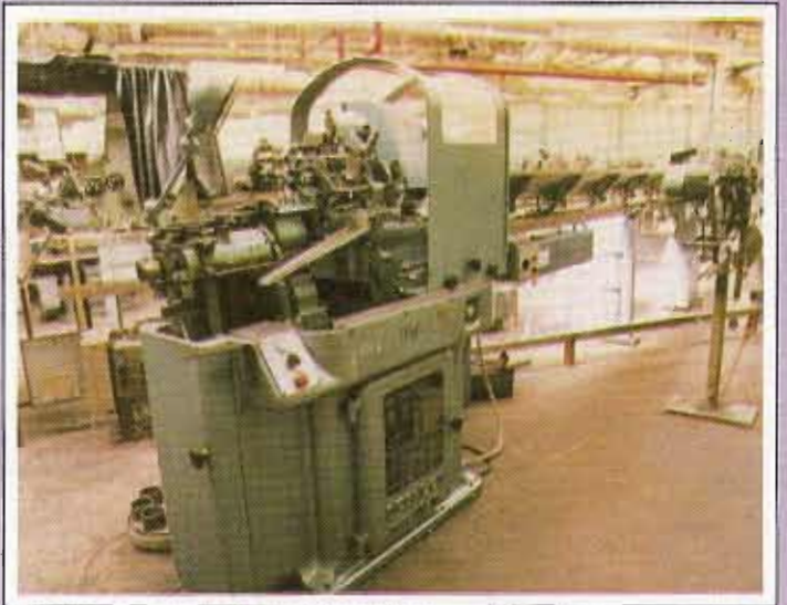
BECHLER ARIO & AR7 (ART (14 machines))
