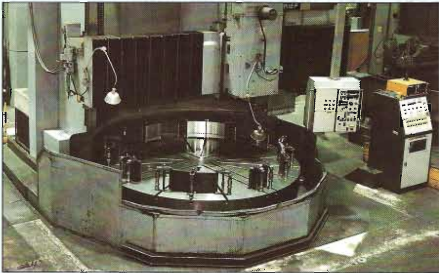
SCHIESS FRORIEP 32 DE 300 N.C. VERTICAL BORER. Table 3000 mm diameter. Swing 3200 mm. Max height 2500 mm. Maximum table loading 20 tons 1-100 rpm.
