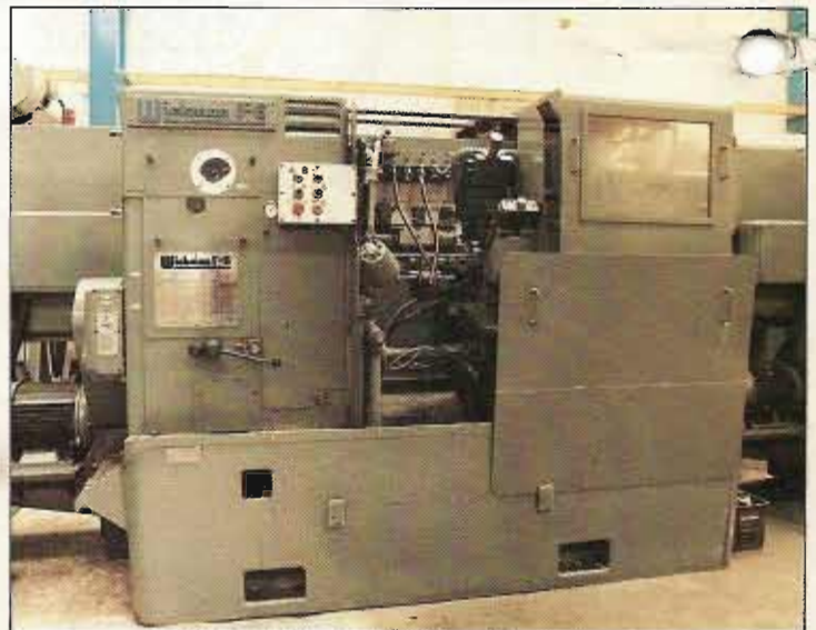
1977 WICKMAN 1" x 6 spindle bar auto
